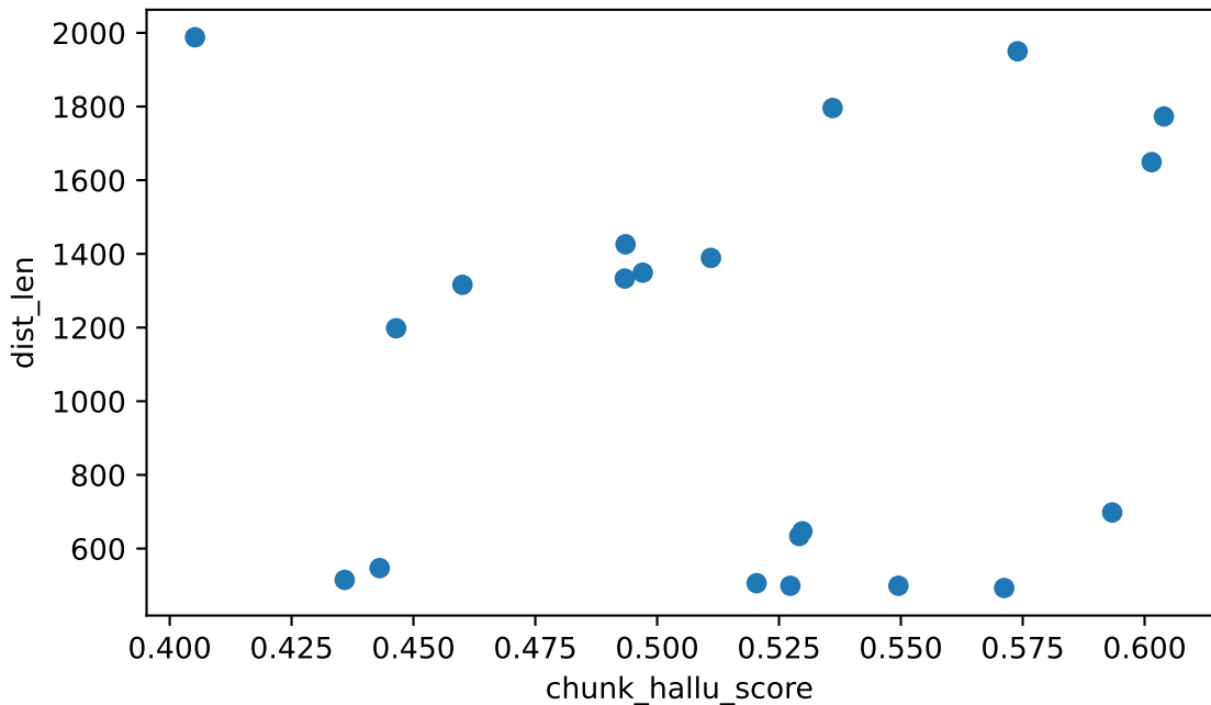
chunk_hallu_score vs dist_len Spearman rho=+0.053 (weak), n=20
