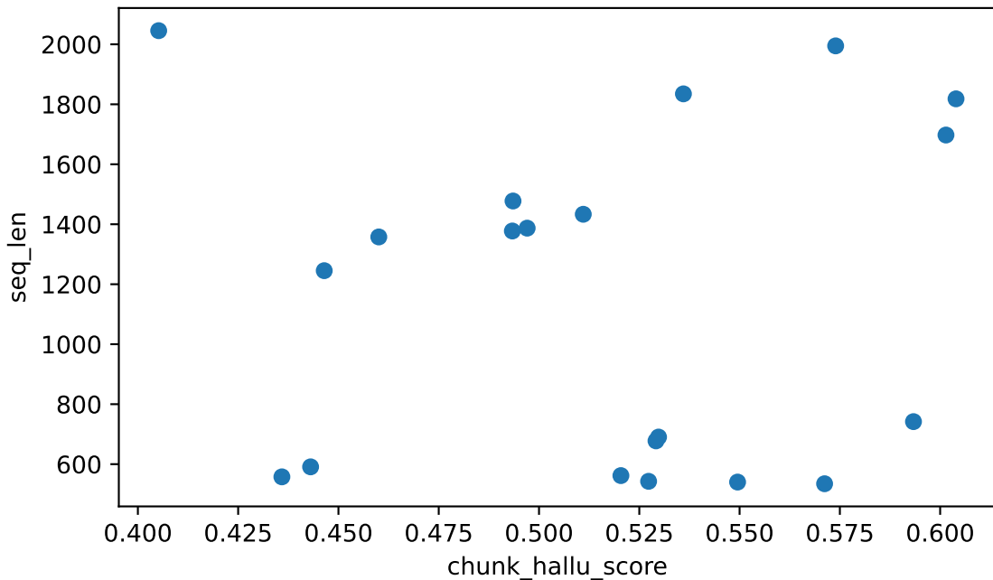
chunk_hallu_score vs seq_len Spearman rho=+0.062 (weak), n=20
