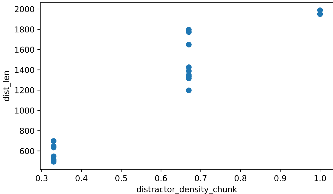
distractor_density_chunk vs dist_len Spearman \rho = +0.905 (strong), n=20
