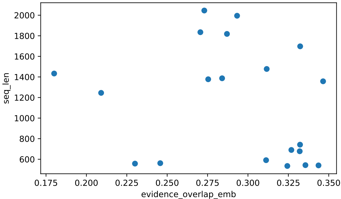
evidence_overlap_emb vs seq_len Spearman rho=-0.292 (weak), n=20
