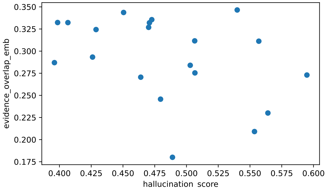
hallucination_score vs evidence_overlap_emb Spearman rho=-0.408 (moderate), n=20
