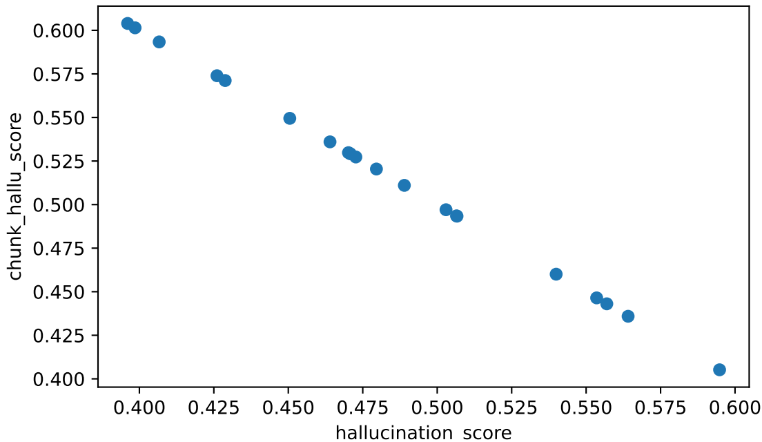
hallucination_score vs chunk_hallu_score Spearman rho=-1.000 (strong), n=20
