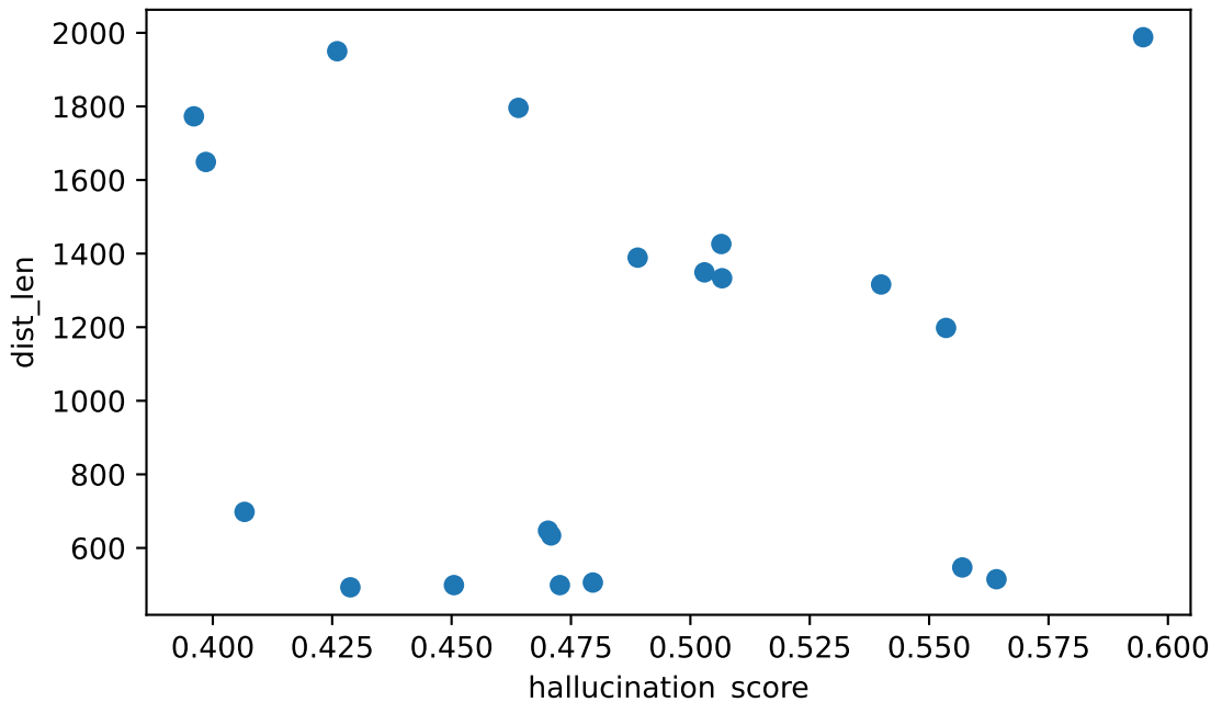
hallucination_score vs dist_len Spearman rho=-0.053 (weak), n=20
