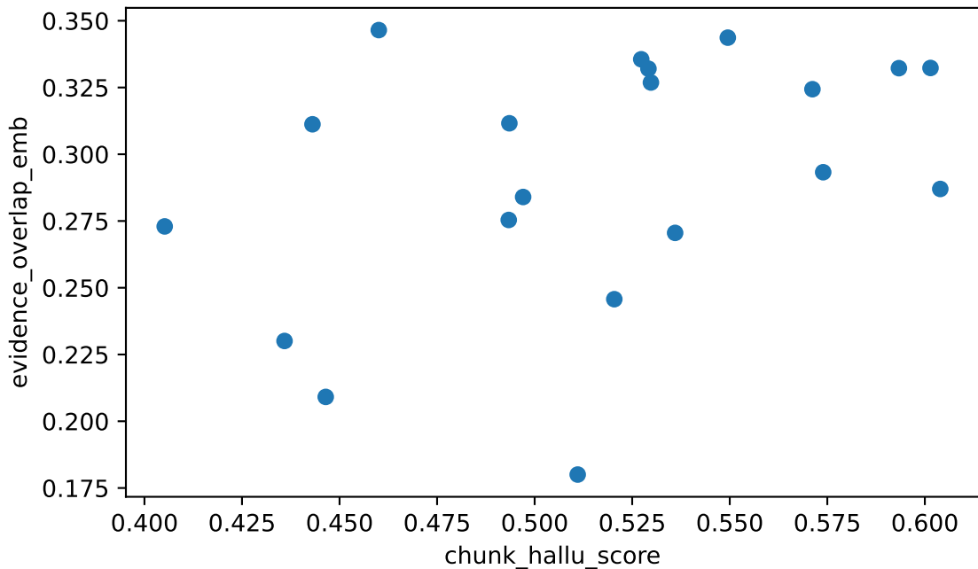
chunk_hallu_score vs evidence_overlap_emb Spearman rho=+0.408 (moderate), n=20
