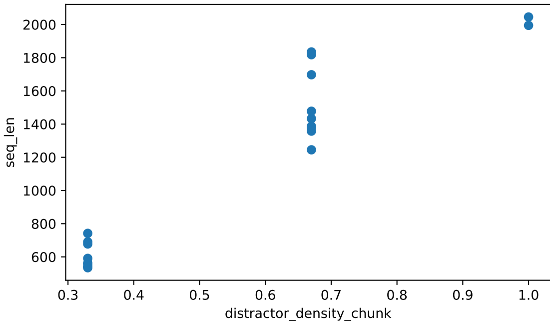
distractor_density_chunk vs seq_len Spearman \rho = +0.905 (strong), n=20
