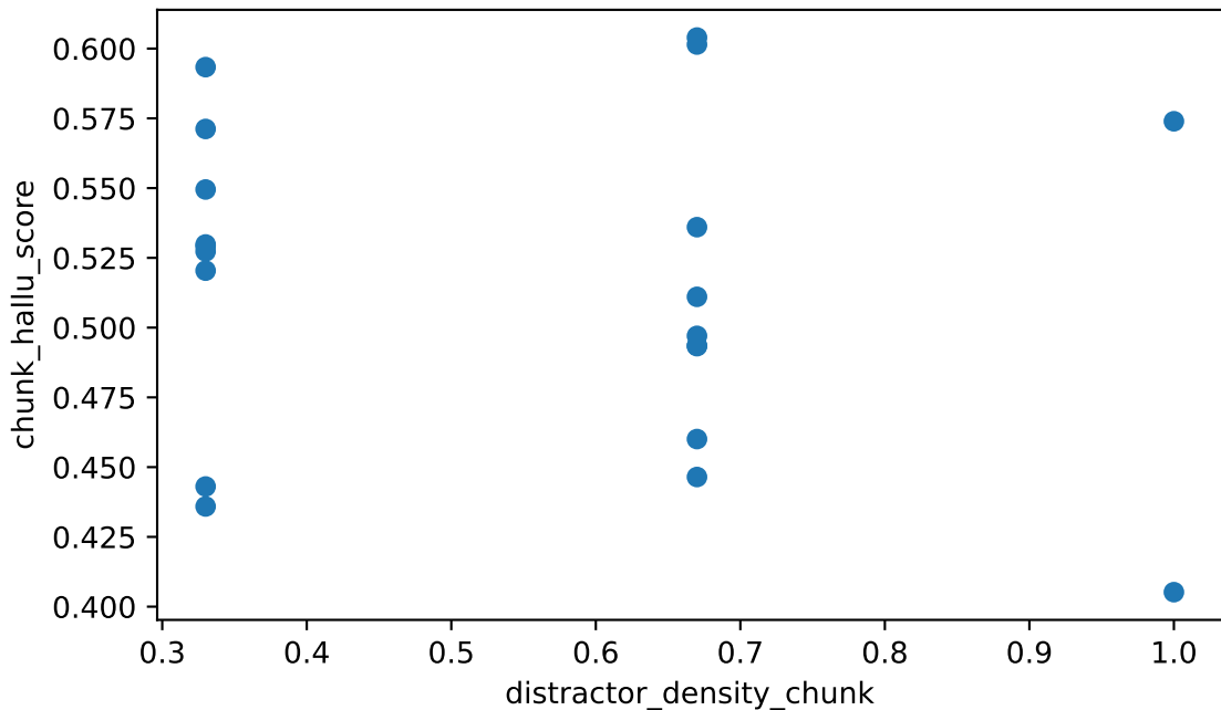
distractor_density_chunk vs chunk_hallu_score Spearman rho=-0.110 (weak), n=20
